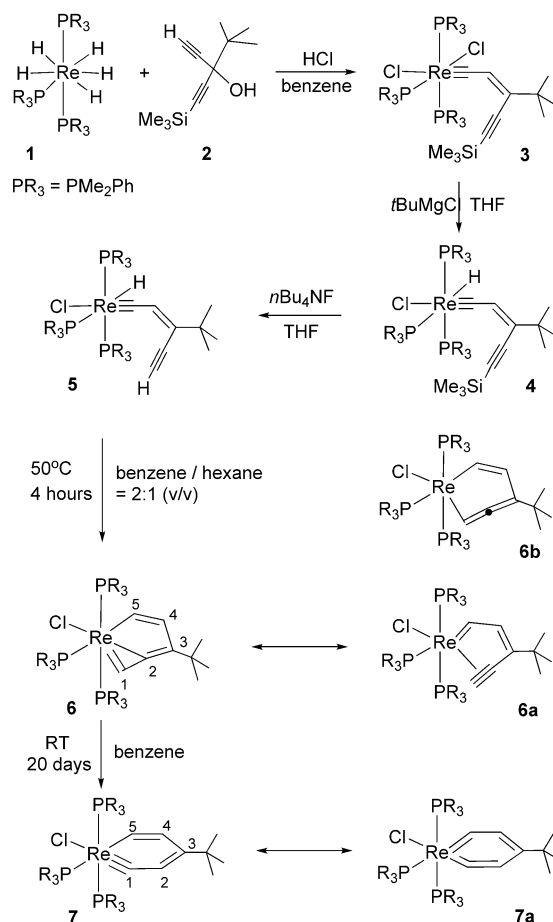
Scheme 1. Preparation of rhenabenzynes 6 and rhenabenzyne 7 .
